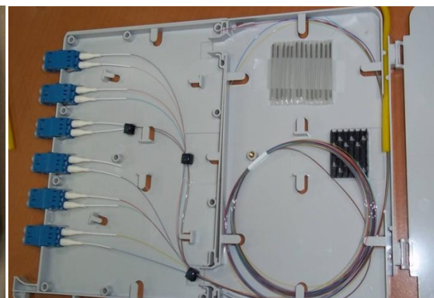
Inner view of 12 fiber/clustered fiber module
